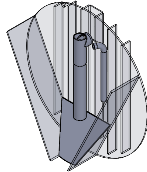
BIOPUHAŞTI SWIRLPIPE SCALE 1:20
