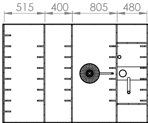
SECTION AA-AA SCALE 1 : 35
